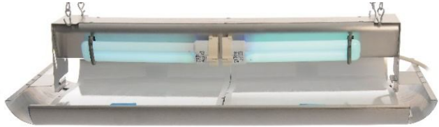
Fly Shield Four showing lighting & glue board arrangement
